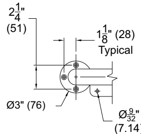
FLANGE DETAIL
