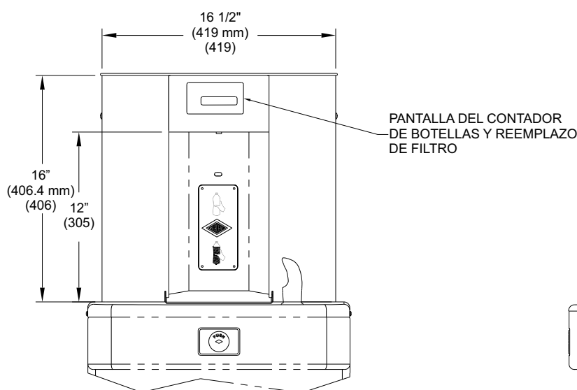
VISTA FRONTAL
